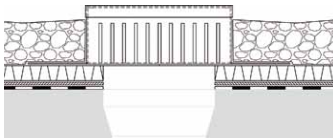
Installation details of inspection chamber
